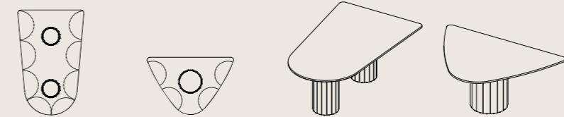
CA610 H 730 L 2000 W 1250 CA620 H 730 L 1200 W 1800 Oregelbunden form Irregular shape Pelare Pedestal Ø 350 Pelare Pedestal Ø 490
