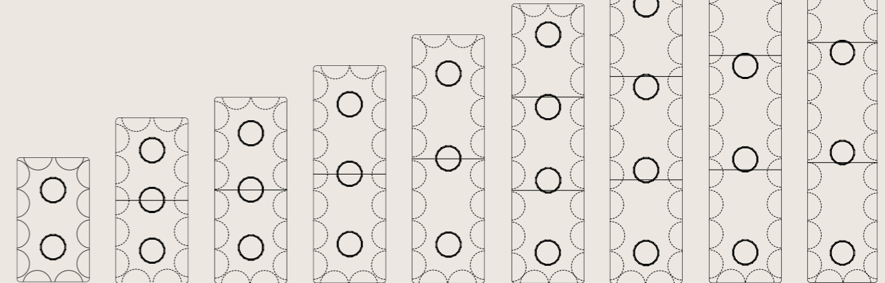
CA1240140 H ** L 2400 W 1400 CA1320140 H ** L 3200 W 1400 CA1360140 H ** L 3600 W 1400 CA1420140 H ** L 4200 W 1400 CA1480140 H ** L 4800 W 1400 CA1540140 H ** L 5400 W 1400 CA1600140 H ** L 6000 W 1400 CA1660140 H ** L 6600 W 1400 CA1720140 H ** L 7200 W 1400
